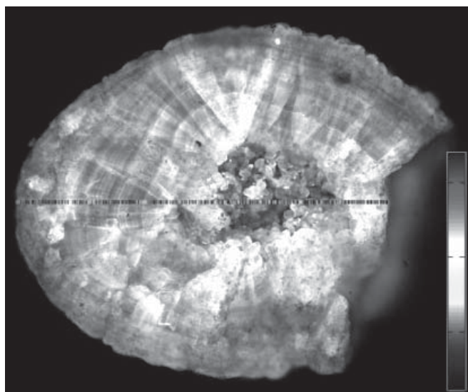
The new diagnostic system makes intermediate postoperative kidney stone analysis possible. Exemplarily, a stone is being analyzed automatically using Raman spectroscopy. (© Fraunhofer IPM) | Picture in color and printing quality: www.fraunhofer.de/press
